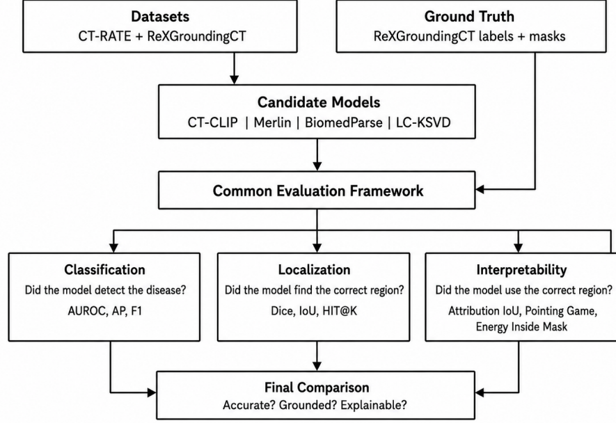
Figure 4.1: Architecture diagram of the proposed evaluation framework.
